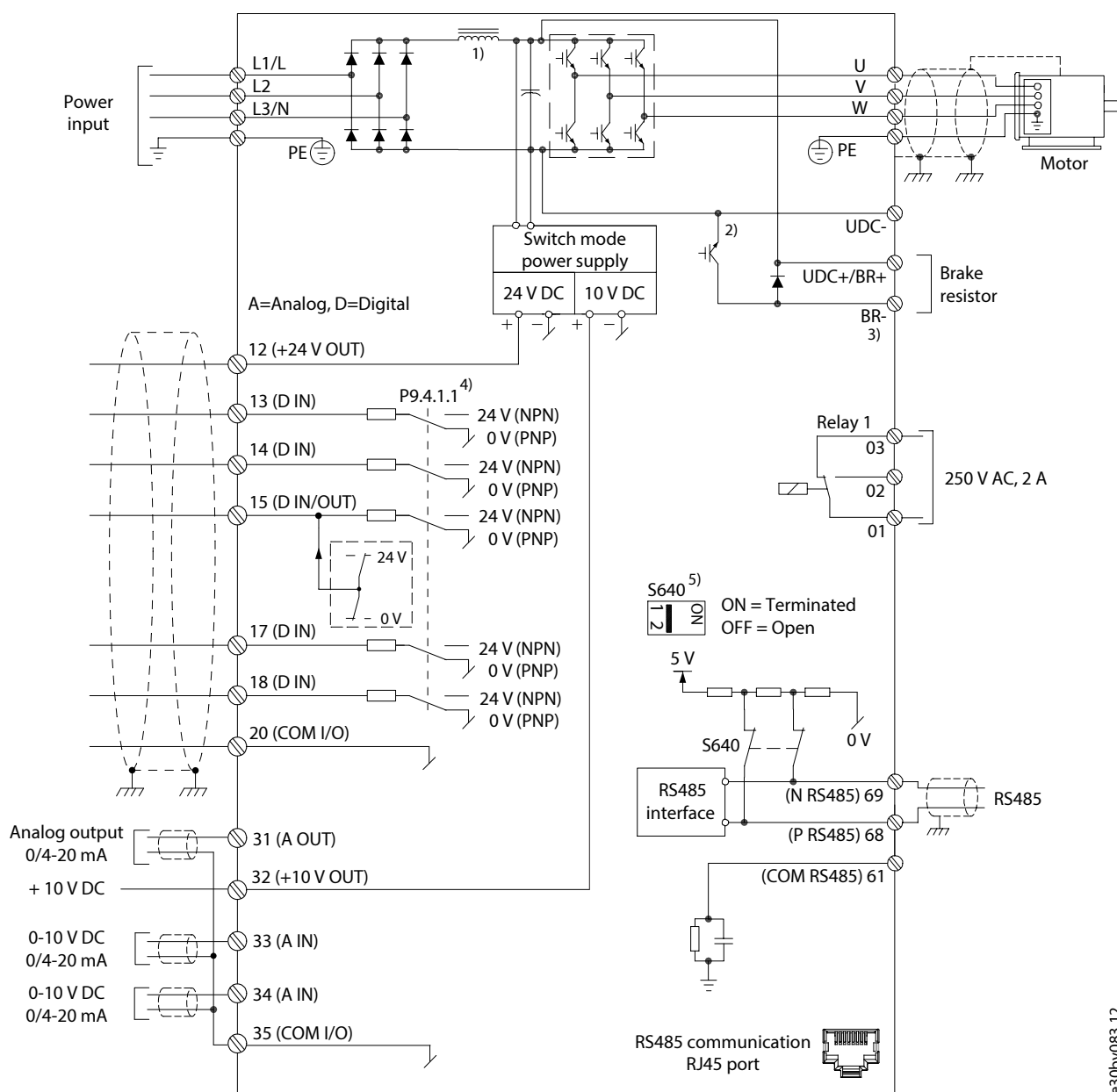
Figure 37: Wiring Diagram
